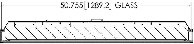
SECTION B-B
